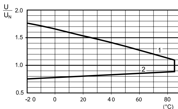
R 40 - AC coil operating range v ambient temperature
