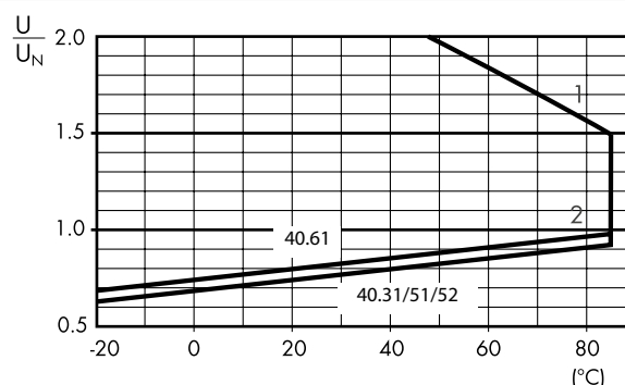
R 40 - DC coil operating range v ambient temperature Sensitive coil, types 40.31/51/52/61
