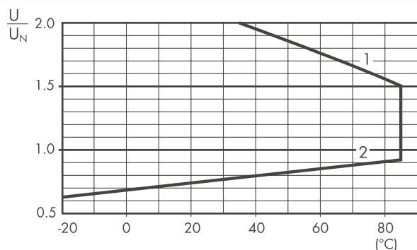
R 40 - DC coil operating range v ambient temperature Standard coil
