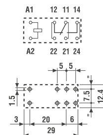
Copper side view Pin length 5.3 mm for PCB or sockets
