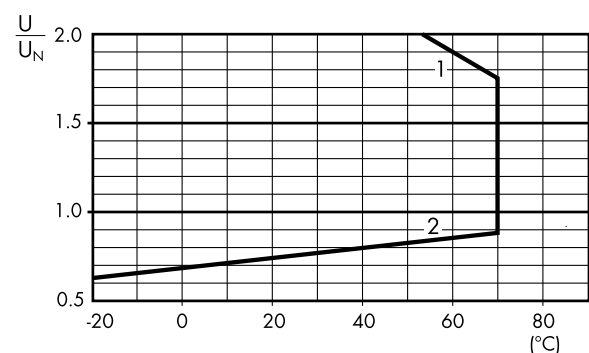
R 40 - DC coil operating range v ambient temperature Sensitive coil, type 40.11
